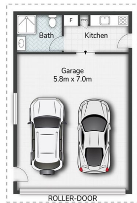
LOWER FLOOR
